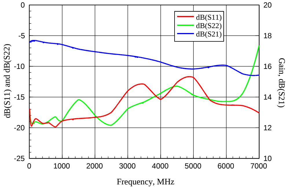
ABL0600-01-1640 Measured Gain and Return Loss vs Frequency
