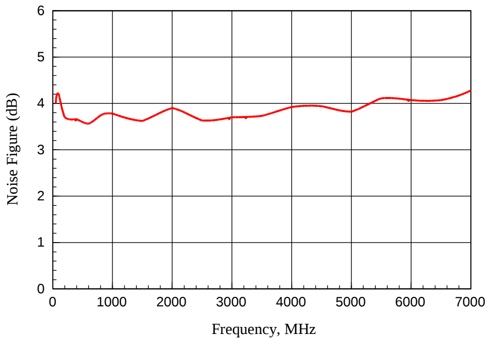
ABL0600-01-1640 Measured Noise Figure vs Frequency
