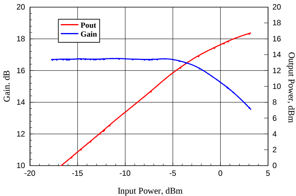
ABL0600-01-1640 Measured Gain and Output Power vs Input Power Test Frequency: 3000MHz
