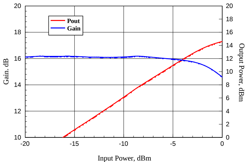
ABL0600-01-1640 Measured Gain and Output Power vs Input Power Test Frequency: 6000MHz
