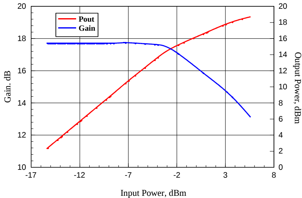
ABL0600-01-1640 Measured Gain and Output Power vs Input Power Test Frequency: 100MHz
